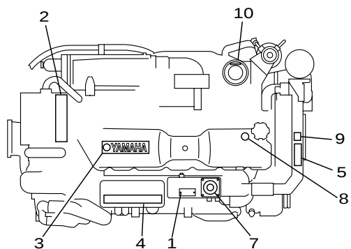
ENGINE UPPER SIDE
